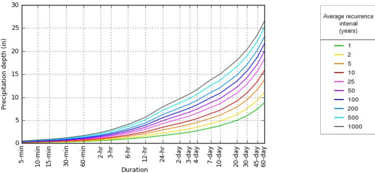
PDS-based depth-duration-frequency (DDF) curves Latitude: 37.7664°, Longitude: -121.7815°
